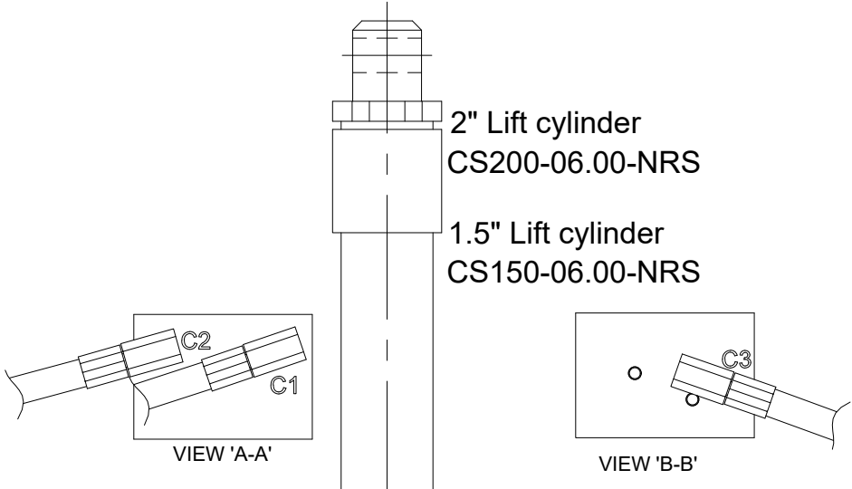
Hydraulic Installation for blades Using M-3493 Power unit
