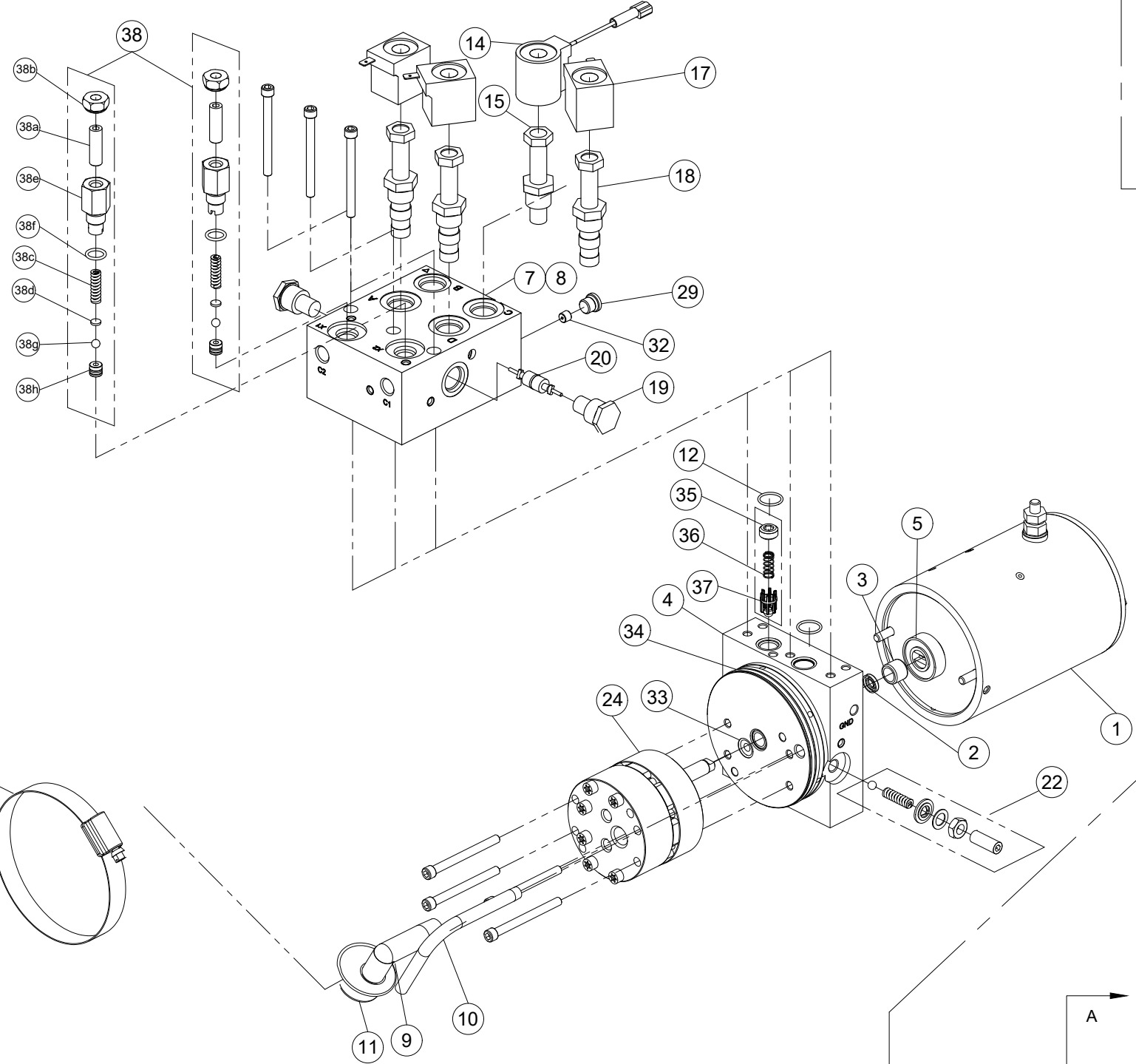
M3493 power unit for Poly & Steel blades
